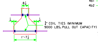
COIL TIE DETAIL NUMBER AND EXACT LOCATION OF COIL TIES TO BE AS DETAILED ON SPECIFIC BRIDGE DESIGN.
