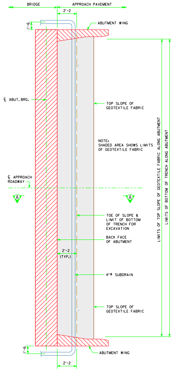
ABUTMENT PLAN WITHOUT WING EXTENSIONS
