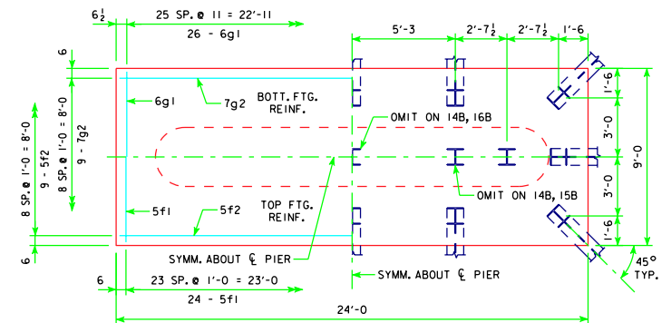
3'-6 x 9'-0 x 24'-0 FOR 14B, 15B & 16B
