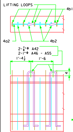
LIFTING LOOP DETAIL ALTERNATE TYPES MAY BE SUBSTITUTED WITH THE APPROVAL OF THE ENGINEER. LIFTING LOOPS ARE TO BE STRUCTURAL GRADE.
