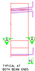
STRAND PROJECTION AT BEAM ENDS WHEN EMBEDDED IN CONCRETE END DIAPHRAGMS
