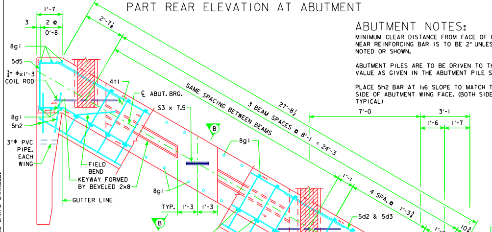
PART REAR ELEVATION AT ABUTMENT
