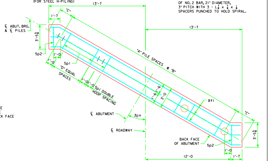
ABUTMENT PILE PLAN
