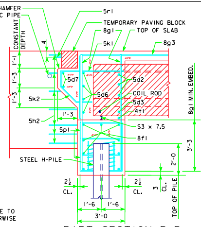
PART SECTION B-B (FOR STEEL H-PIILING)
