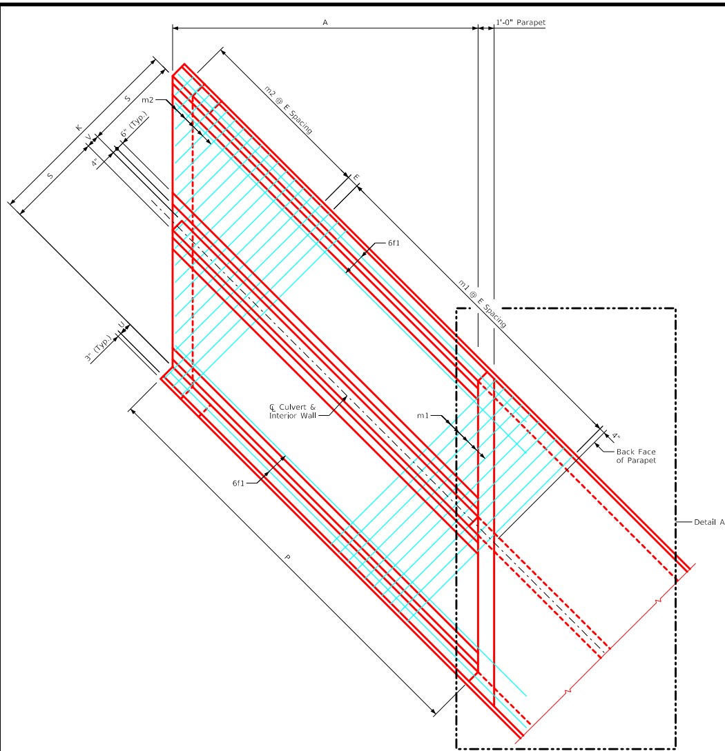
Plan View - Top Apron Reinforcing (Wall Reinforcing not shown for clarity)
