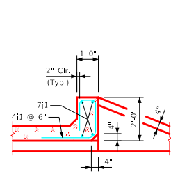
Section thru Parapet
