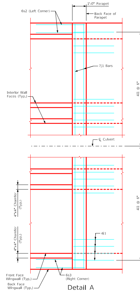
Detail A (Showing parapet bars only)
