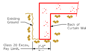
Curtain Wall Class 20 Excavation
