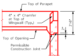
Top of Wingwall Details
