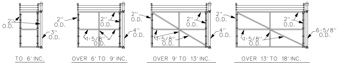
FRAME PATTERNS FOR VARIOUS GATE OPENINGS
