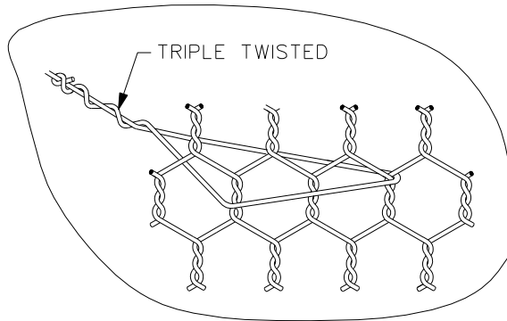
GABION WALLS
