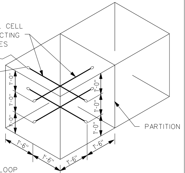
TYPICAL INTERIOR BASKET WIRING DETAIL
