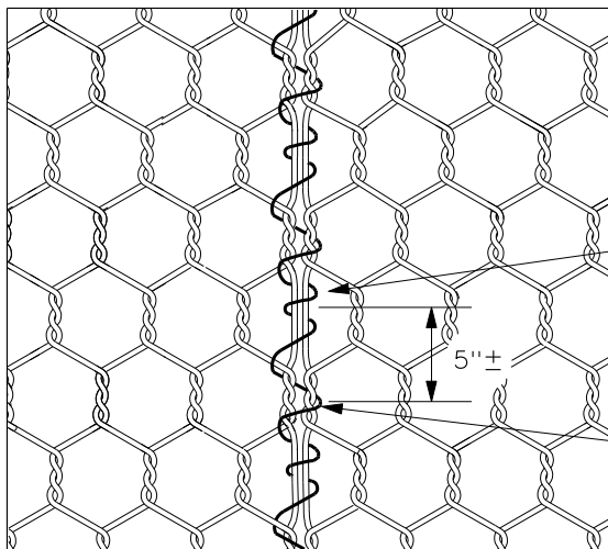
LACING DIAGRAM
