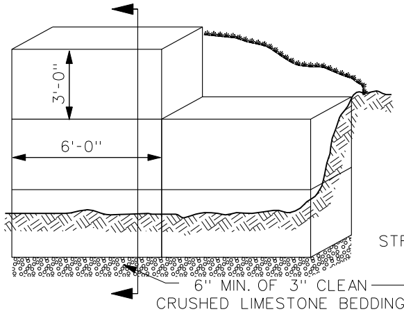
GABION WALLS
