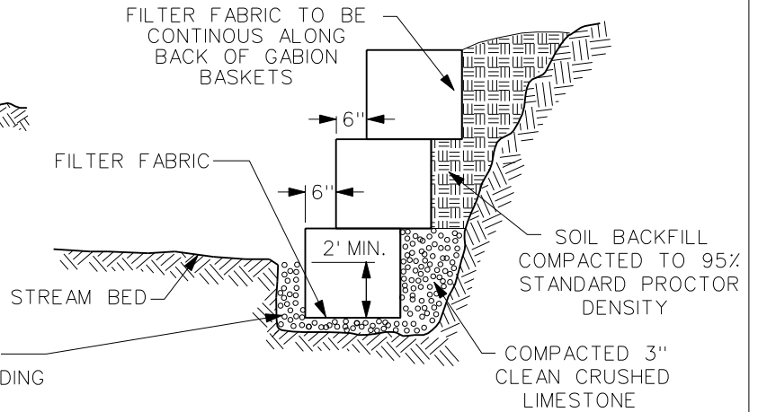
SECTION Y-Y
