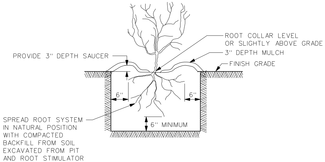
BARE ROOT PLANTING PIT
