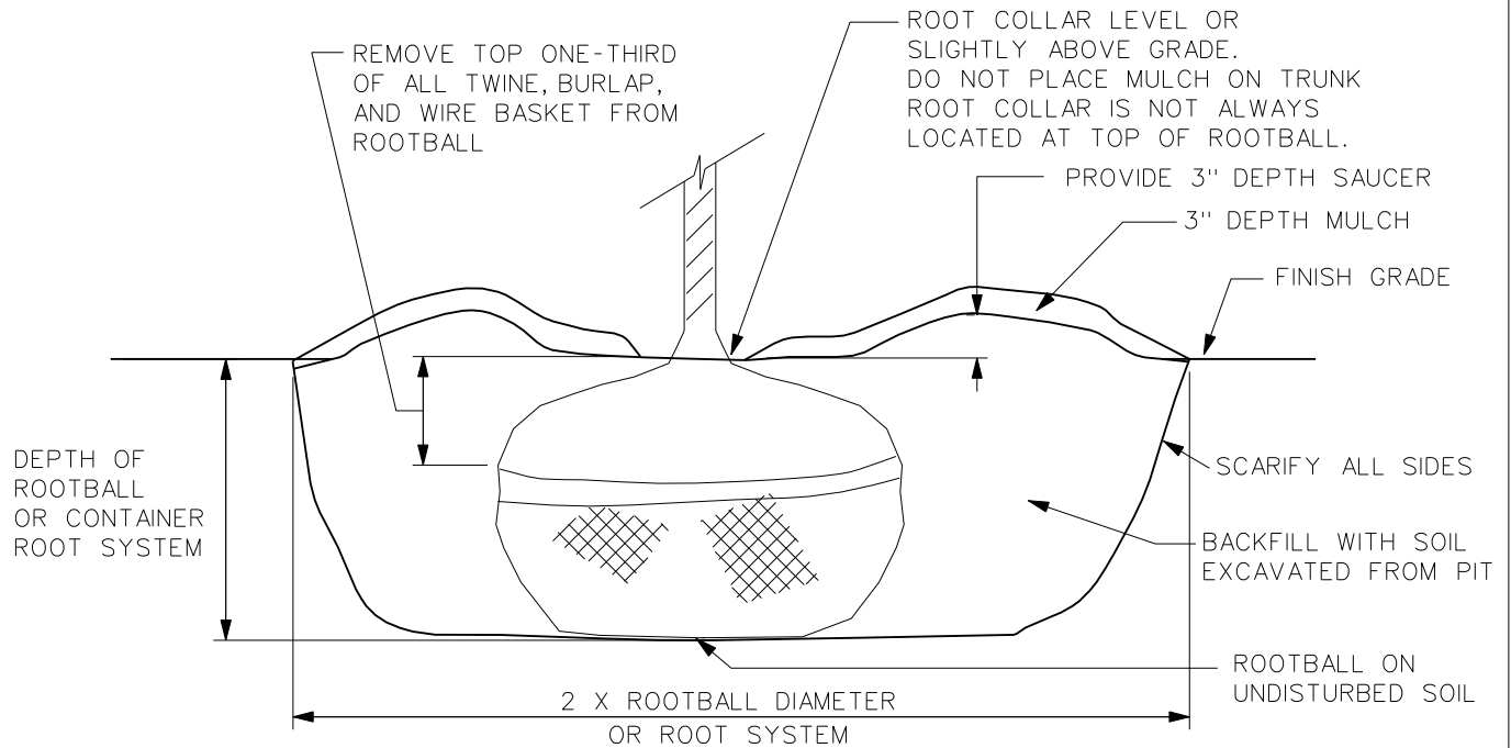
TYPICAL PLANTING PIT
