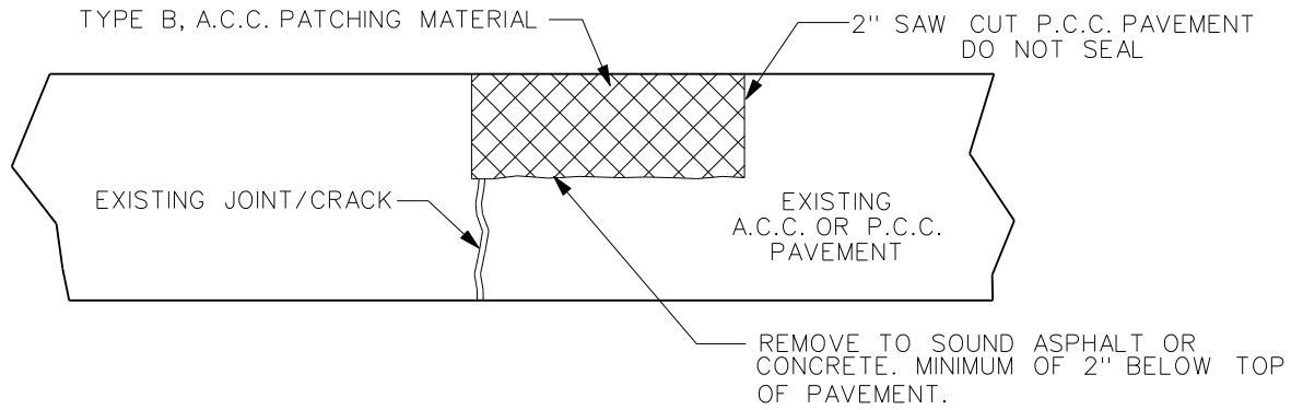
PARTIAL DEPTH A.C.C. PATCH
