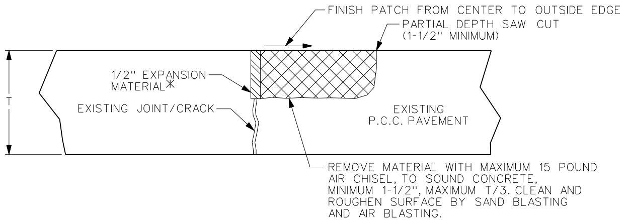
TYPE A PARTIAL DEPTH P.C.C. PATCH
