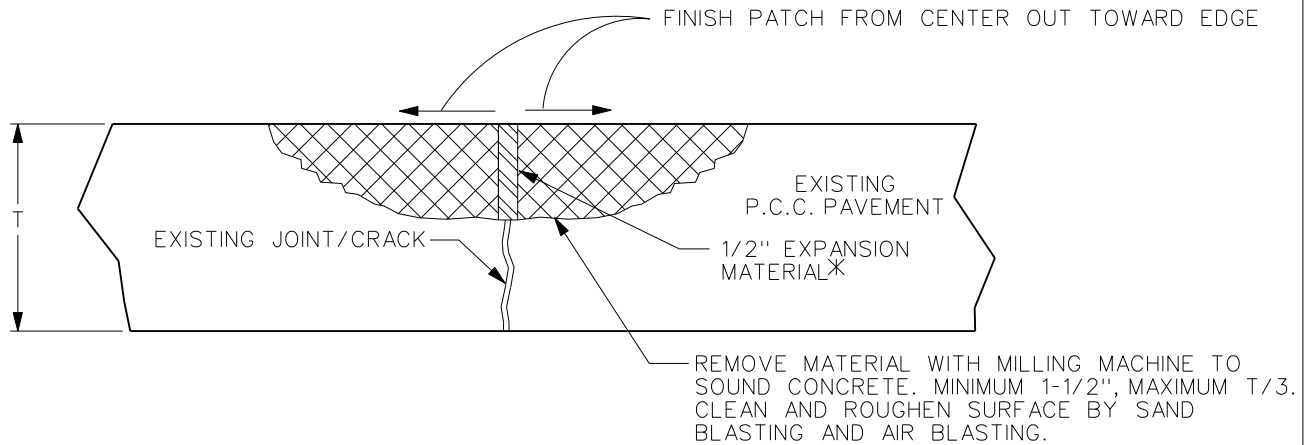
TYPE B PARTIAL DEPTH P.C.C. PATCH
