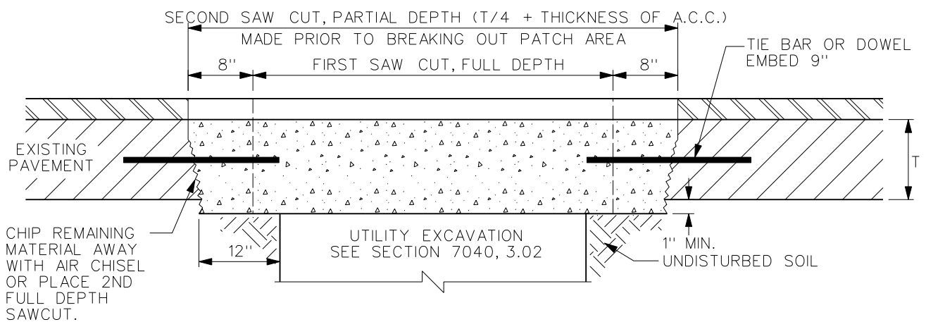
P.C. CONCRETE FULL DEPTH PATCH (COMPOSITE SECTION)
