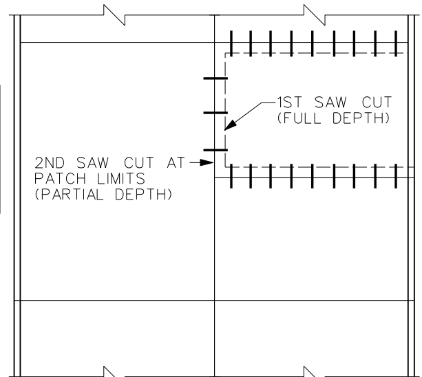
PAVEMENT PLAN
