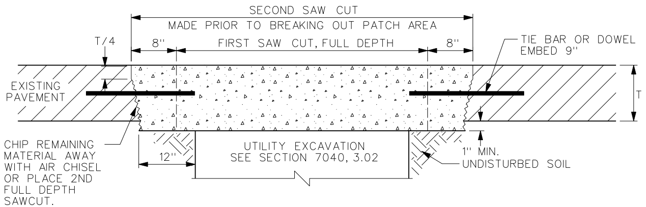
P.C. CONCRETE FULL DEPTH PATCH
