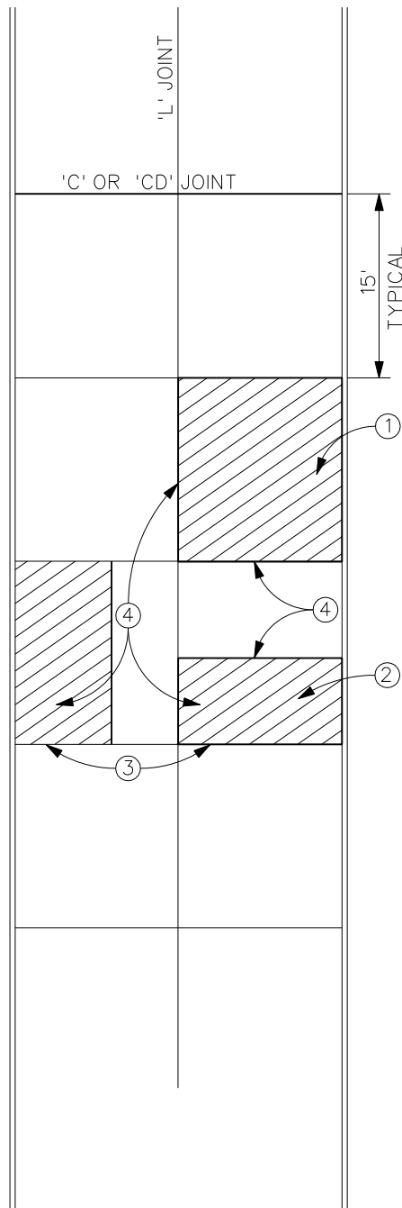
MINIMUM PATCH REQUIREMENTS FOR P.C.C. PAVEMENT
