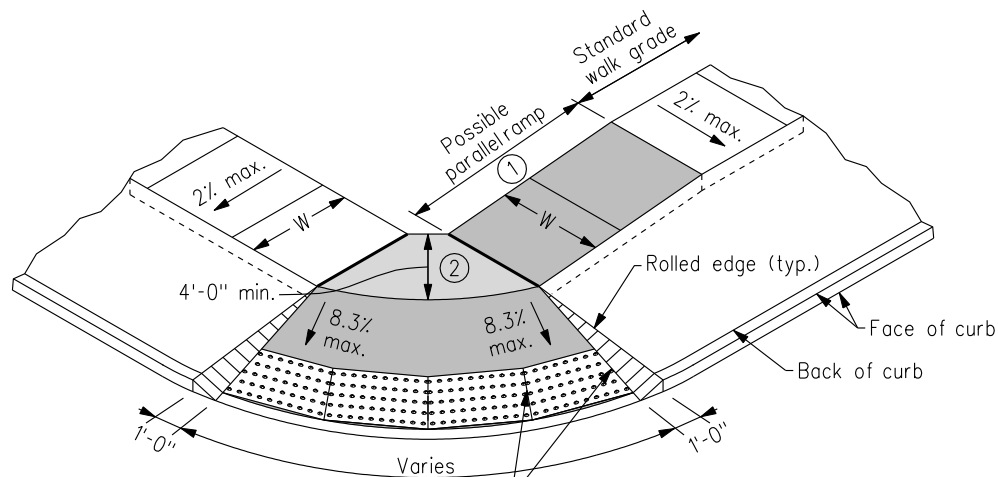
ALTERNATE RAMP 1
