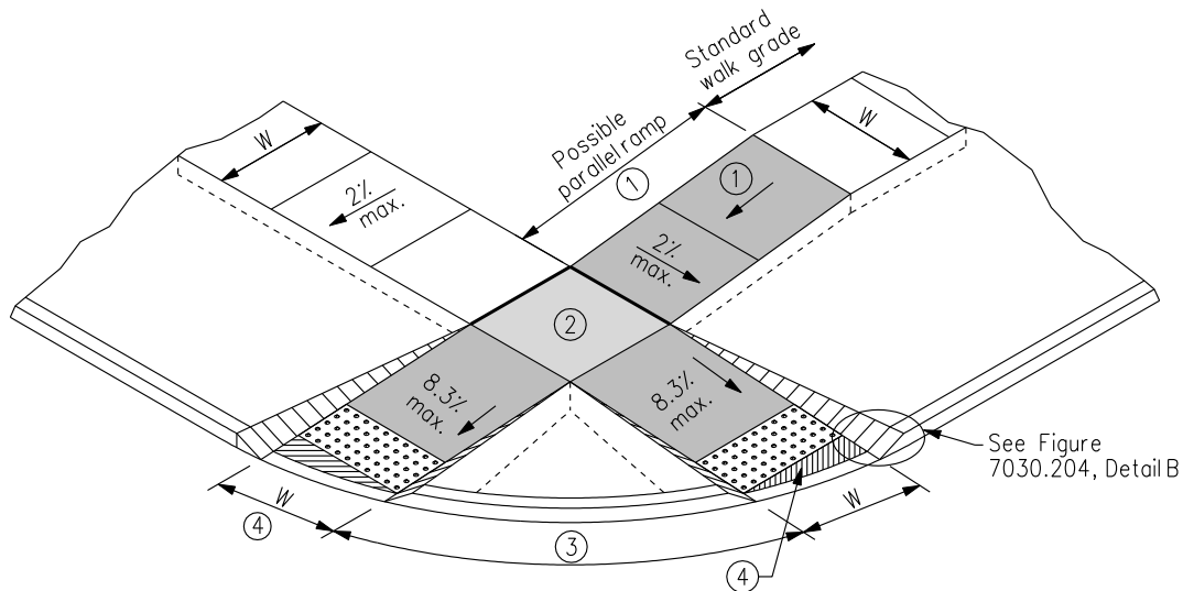
ALTERNATE RAMP 1
