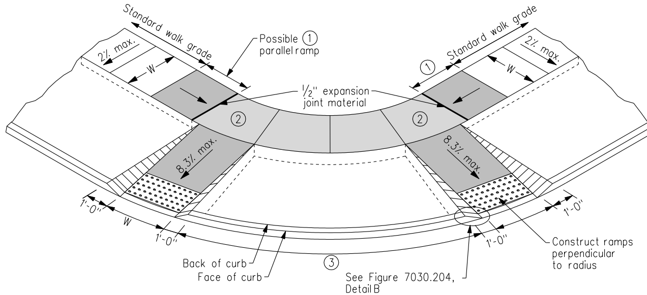
PREFERRED RAMP
