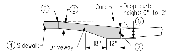
TYPICAL SECTION
