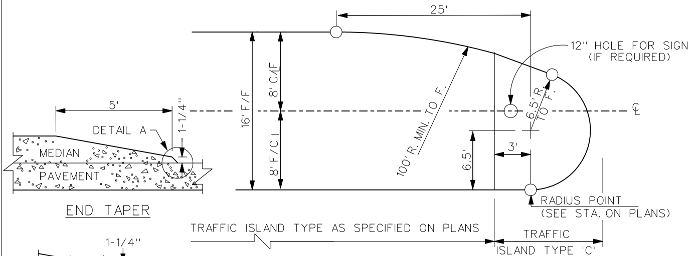
TRAFFIC ISLAND NOSE TYPE II
