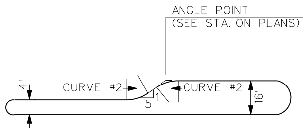
TRAFFIC ISLAND CURVE DETAILS
