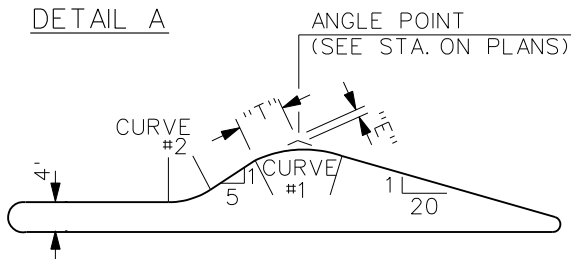
TRAFFIC ISLAND CURVE DETAILS
