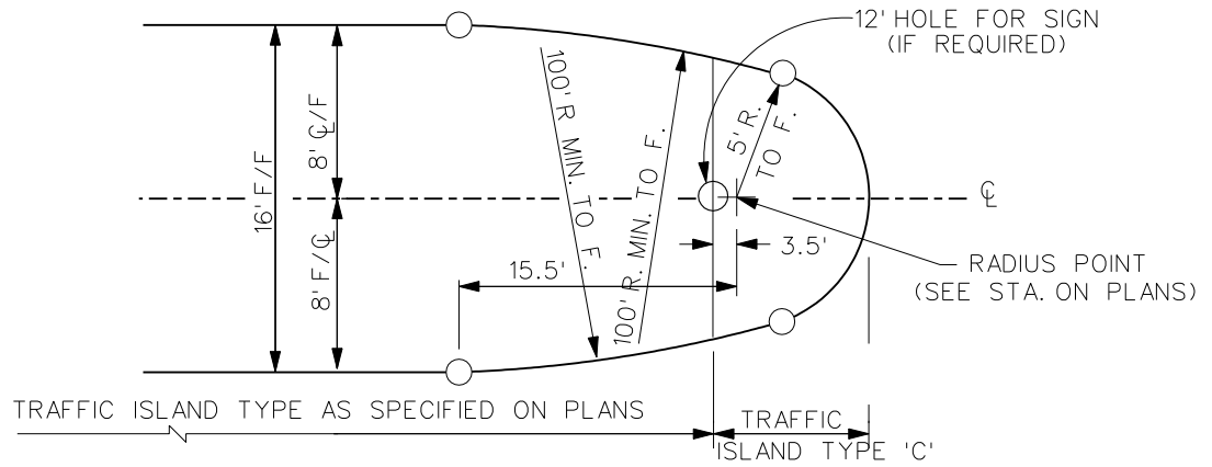
TRAFFIC ISLAND NOSE TYPE I
