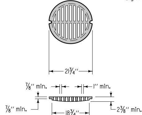
GRATE ①
