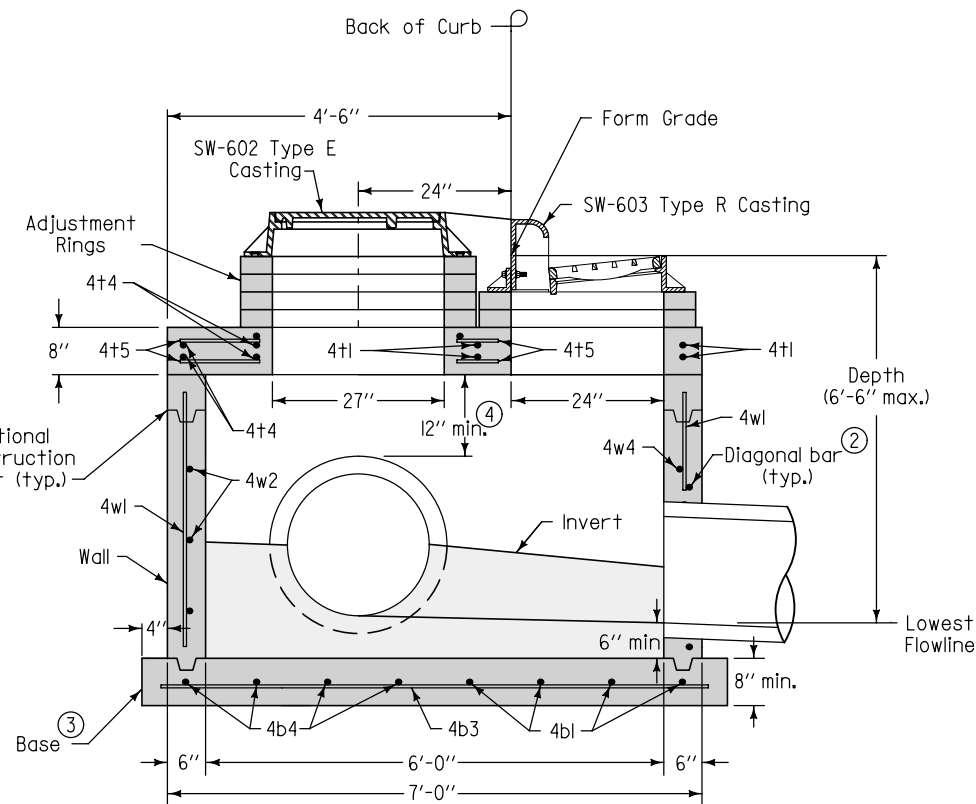
SECTION B-B
