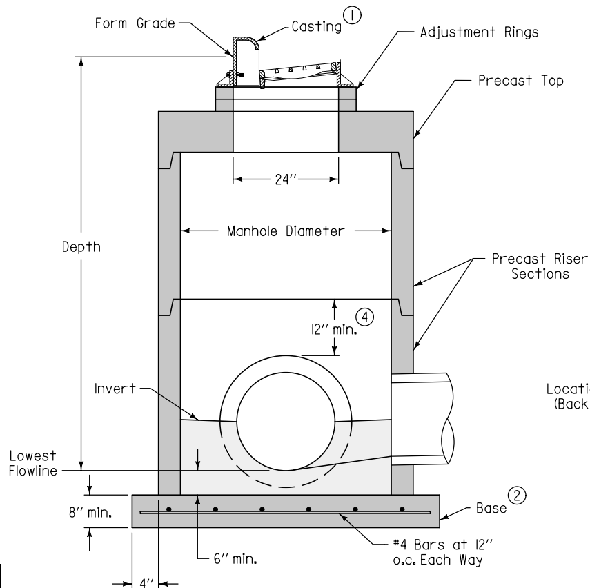
TYPICAL SECTION
