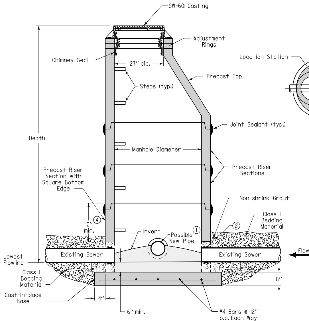
TYPICAL SECTION
