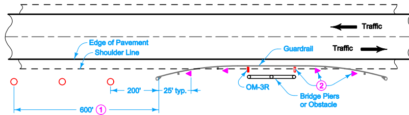
TYPE 4 MARKING SIDE OBSTACLES (STEEL BEAM GUARDRAIL ON THE SHOULDER)
