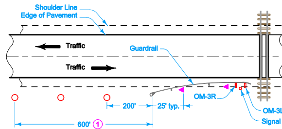
TYPE 8 MARKING RAILROAD CROSSING SIGNALS (TWO-WAY TRAFFIC)
