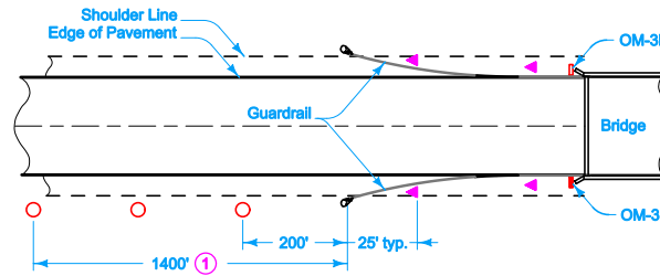
TYPE 1 BRIDGE OR CONCRETE BARRIER RAIL (LESS THAN FULL SHOULDER WIDTH AND BRIDGE/ROADWAY WIDTH LESS THAN 30 FT.)
