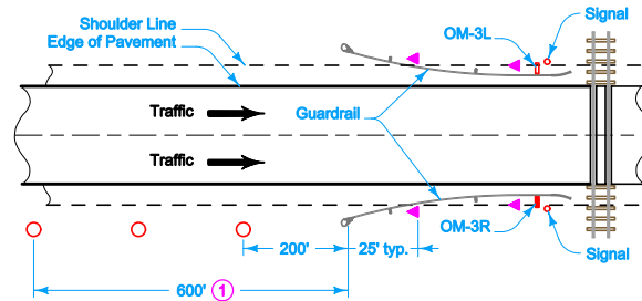
TYPE 7 MARKING RAILROAD CROSSING SIGNALS (ONE-WAY TRAFFIC)
