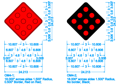
END OF ROADWAY MARKER FABRICATION
