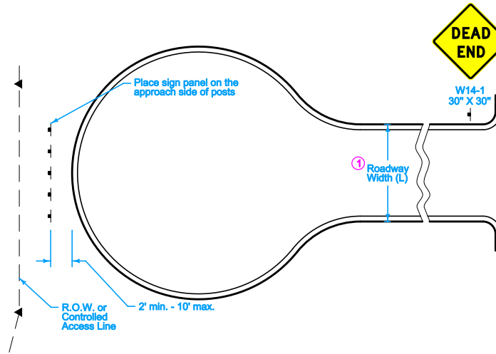
DEAD END WITH CUL-DE-SAC
