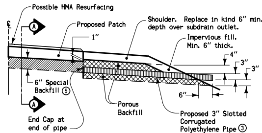
SPECIAL BACKFILL AND SUBDRAIN
