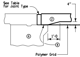
DETAIL 'A' Movable Abutment Bridge
