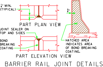
BARRIER RAIL JOINT DETAILS
