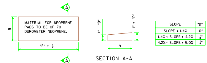
PLAN OF NEOPRENE PAD
