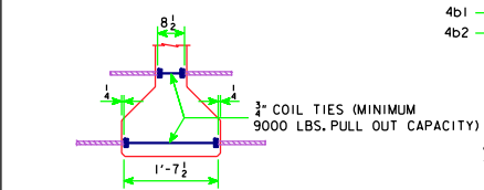
COIL TIE DETAIL NUMBER AND EXACT LOCATION OF COIL TIES TO BE AS DETAILED ON SPECIFIC BRIDGE DESIGN.
