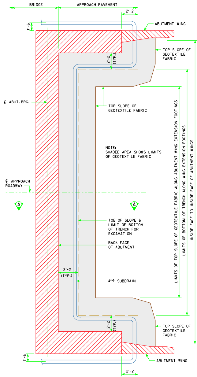
ABUTMENT PLAN WITH WING EXTENSIONS
