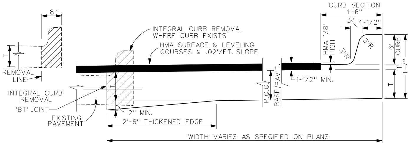
TYPICAL SECTION
