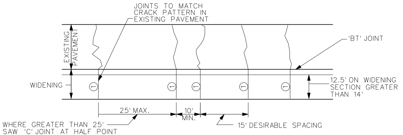
TYPICAL JOINT LAYOUT
