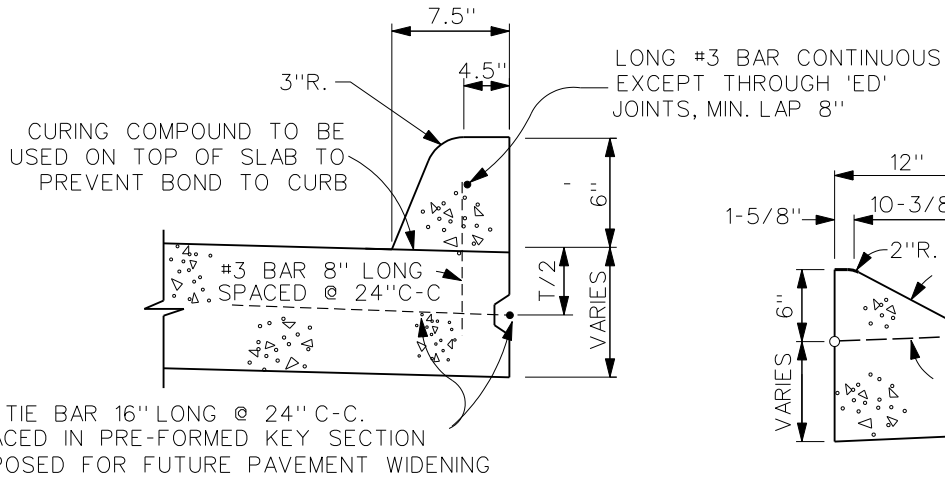
INTEGRAL 6" SLOPED CURB
