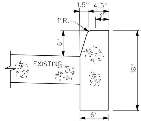
BEAM CURB*
