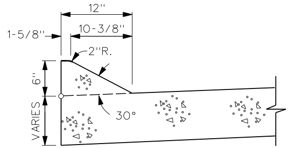
INTEGRAL 6" SLOPED CURB
