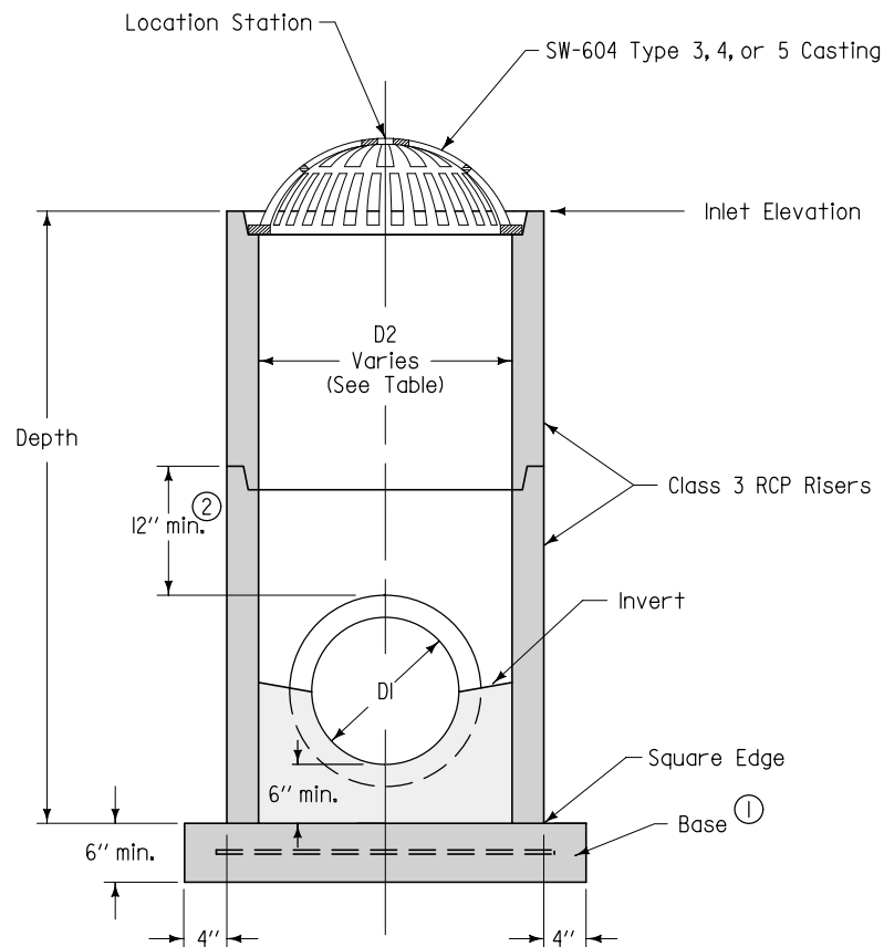
TYPICAL SECTION
