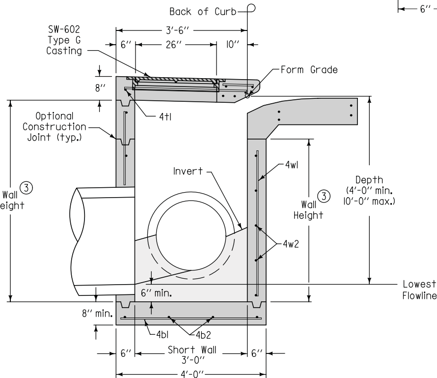
TYPICAL SECTION
