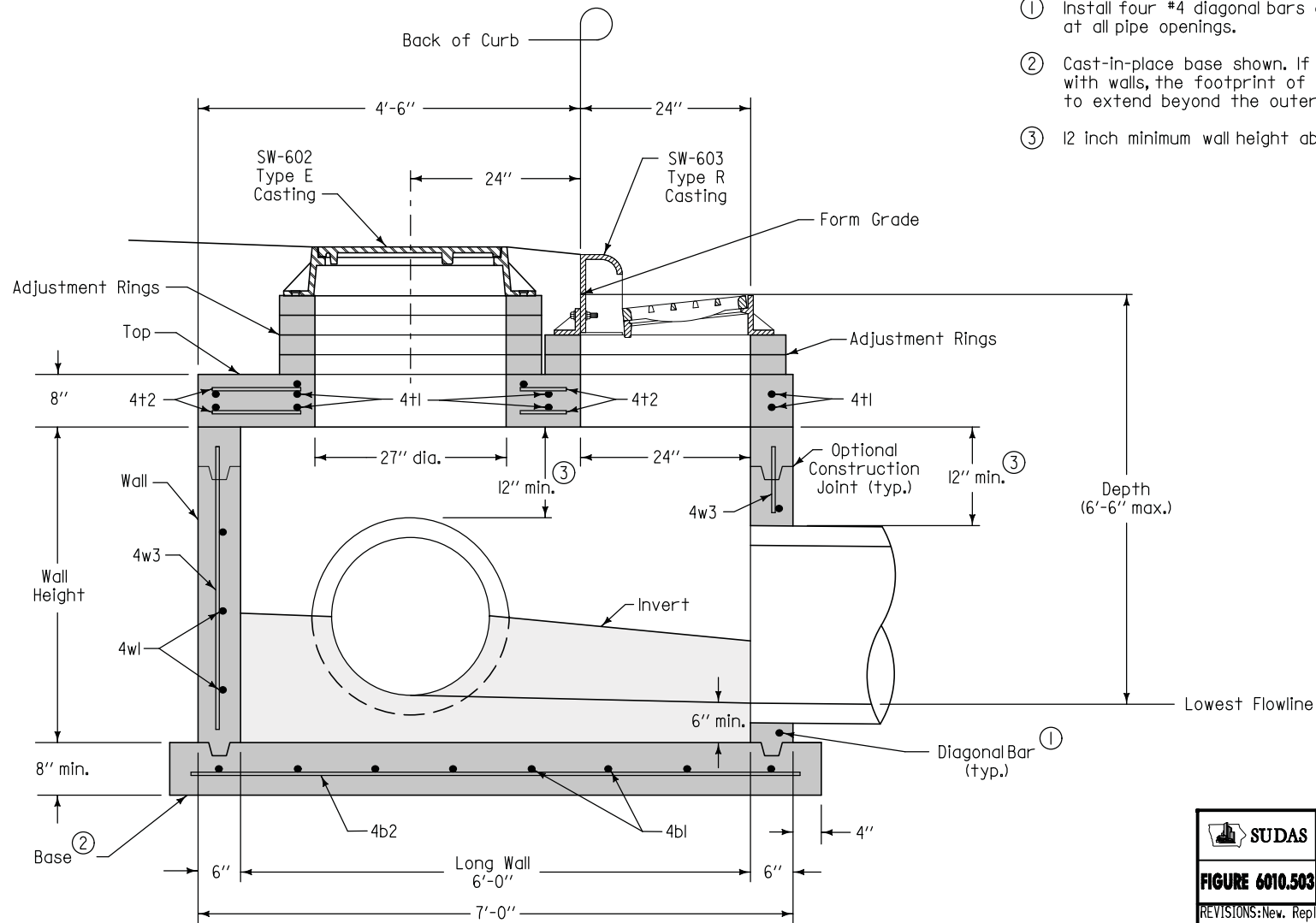
TYPICAL SECTION
