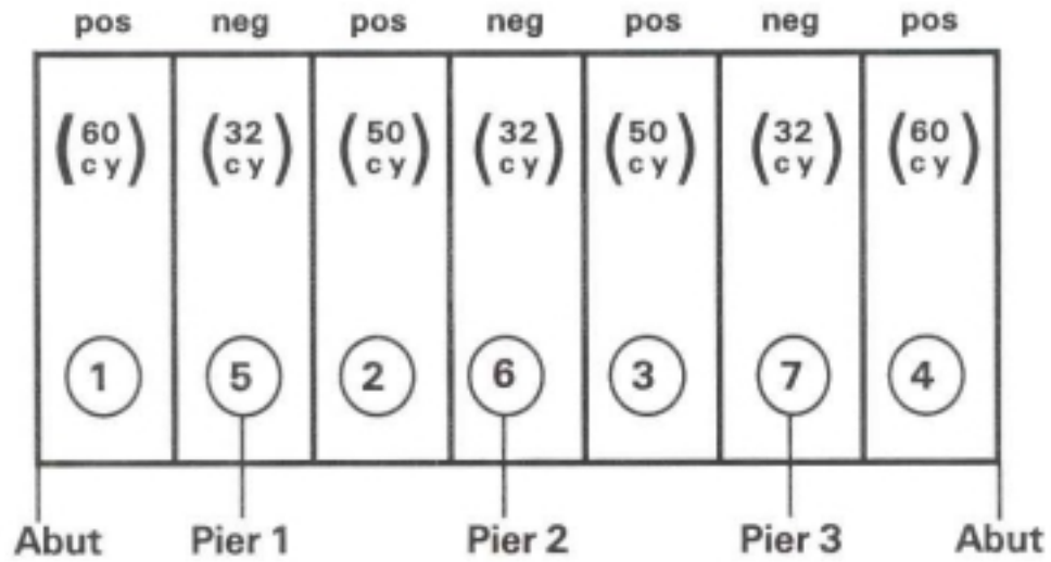
EXAMPLE CONCRETE PLACEMENT DIAGRAM 1 (Noncontinuous)
