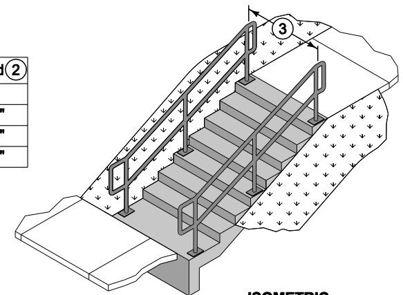
ISOMETRIC
