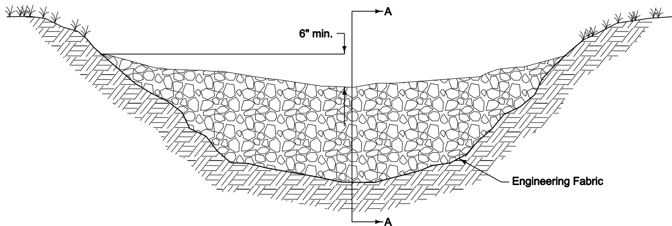
DITCH CROSS-SECTION
