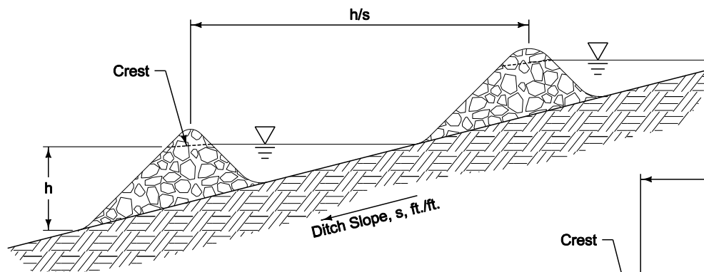
ROCK CHECK DAM (See Figure 9040.7 for installation of Rock Check Dams.)
