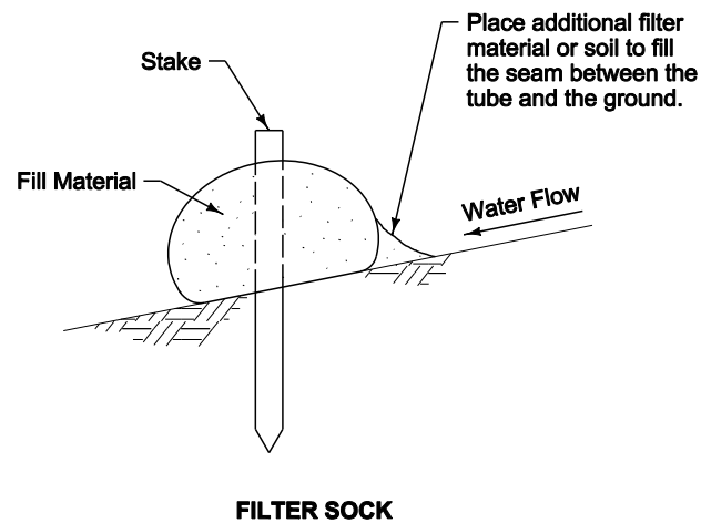
TYPICAL PLACEMENT OF BERM OR SOCK
