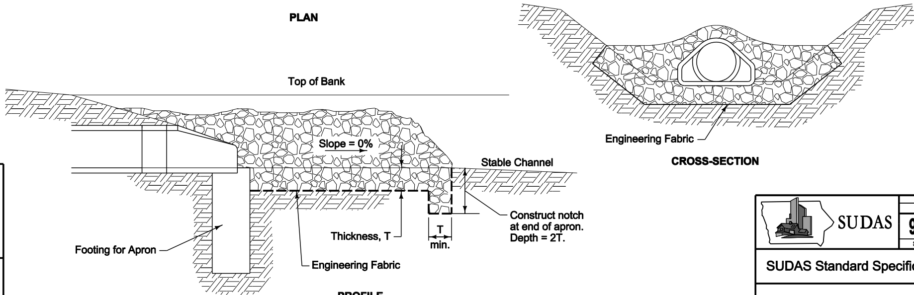
PROFILE Section A-A
