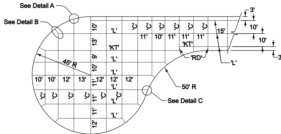
GUTTERLINE JOINTING
