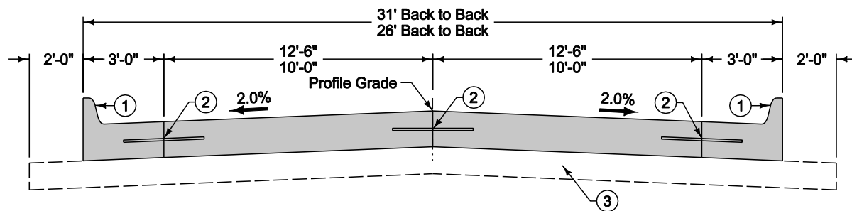
GUTTERLINE JOINTING
