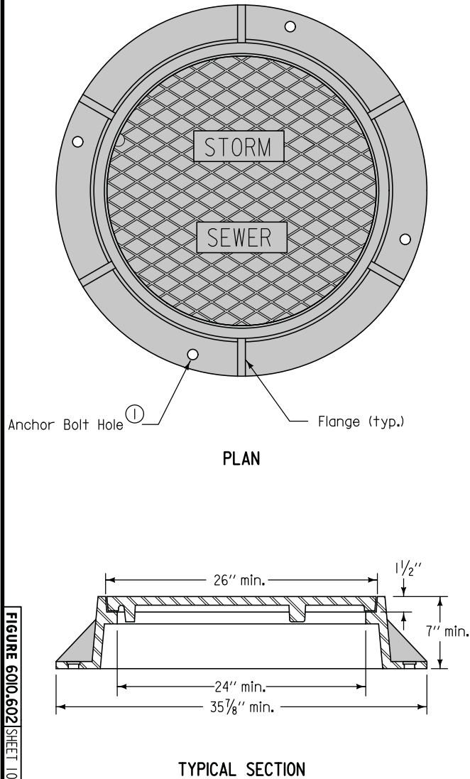
TYPE E Two-piece fixed casting
