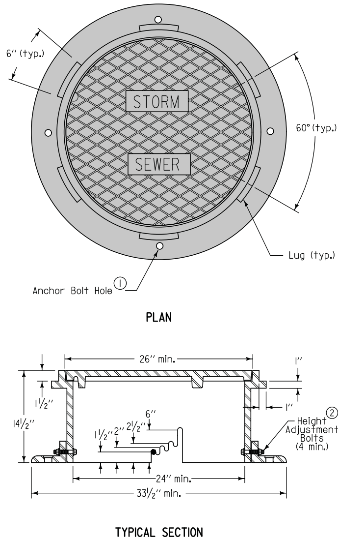
TYPE F Three-piece floating casting
