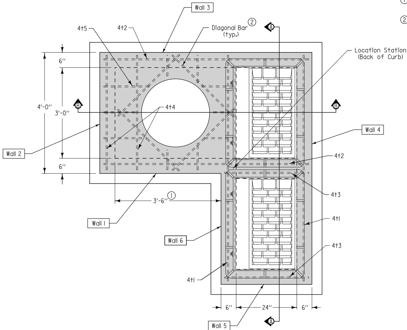
PLAN
