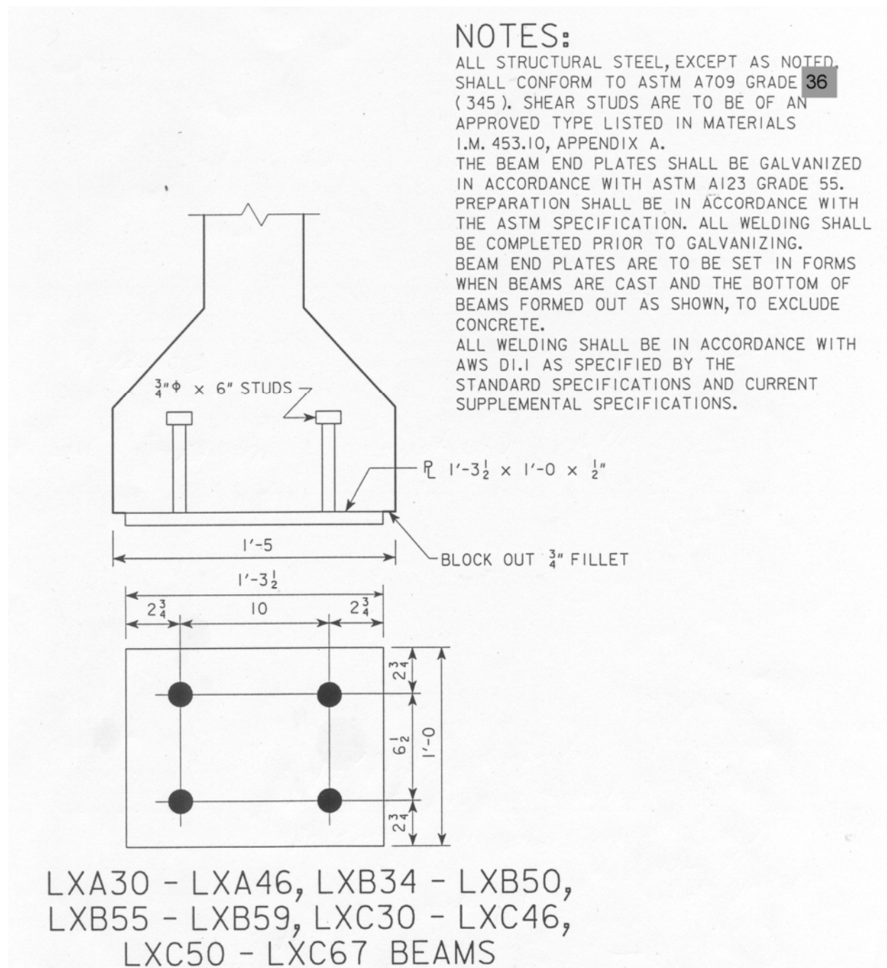
Figure 1. - Optional Beam Seat Protection Plate
