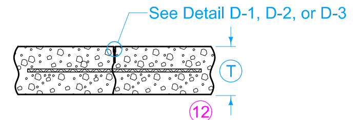
'L' CONTRACTION JOINT
