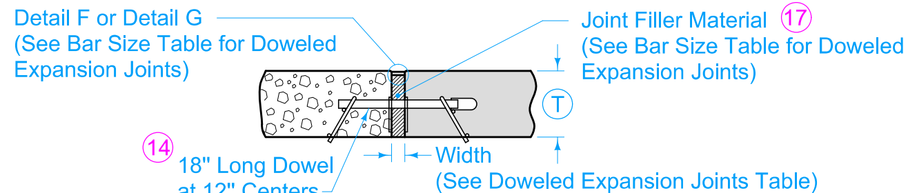
'ED', 'EE', 'EF' JOINT DOWELED EXPANSION JOINT
