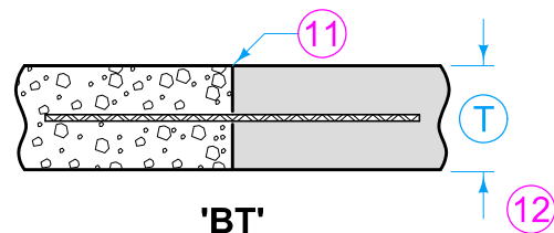
'B' PLAIN JOINT (Abutting Pavement Slabs)
