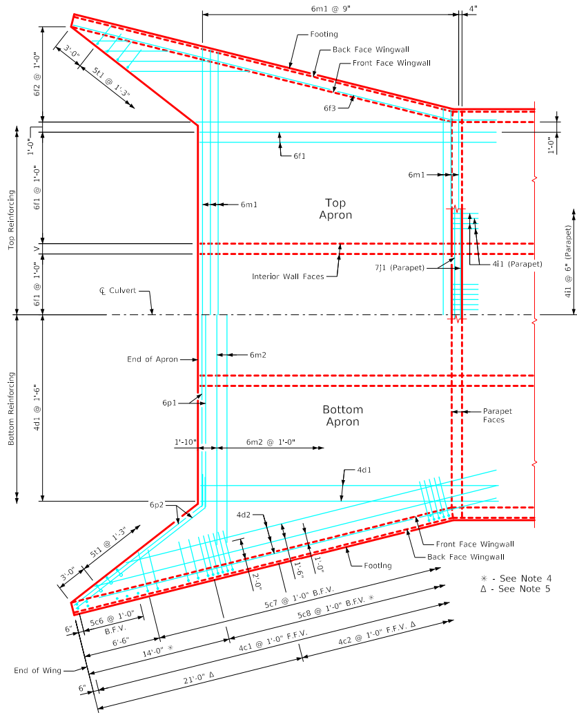
Plan View - Top & Bottom of Apron Reinforcing
