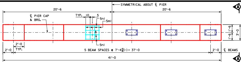
TYPICAL PLAN
