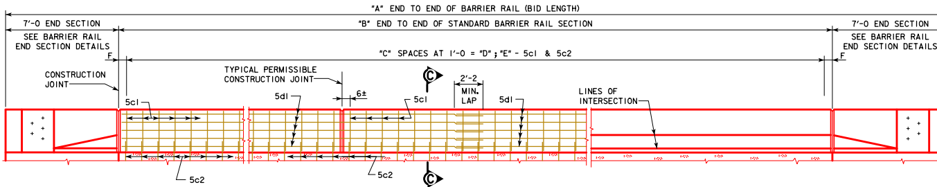
ELEVATION OF BARRIER RAIL LAYOUT
